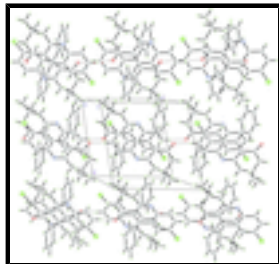
Fig. 2. The crystal packing of the title compound, viewed approximately along the a axis, showing extended one-dimensional chains. The intermolecular interactions are shown as dashed lines.
